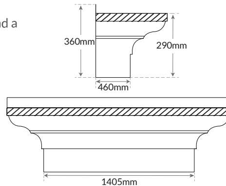
Picture shown with BRG12 brackets
